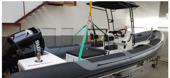
CENTRE POINT LIFT (17)
